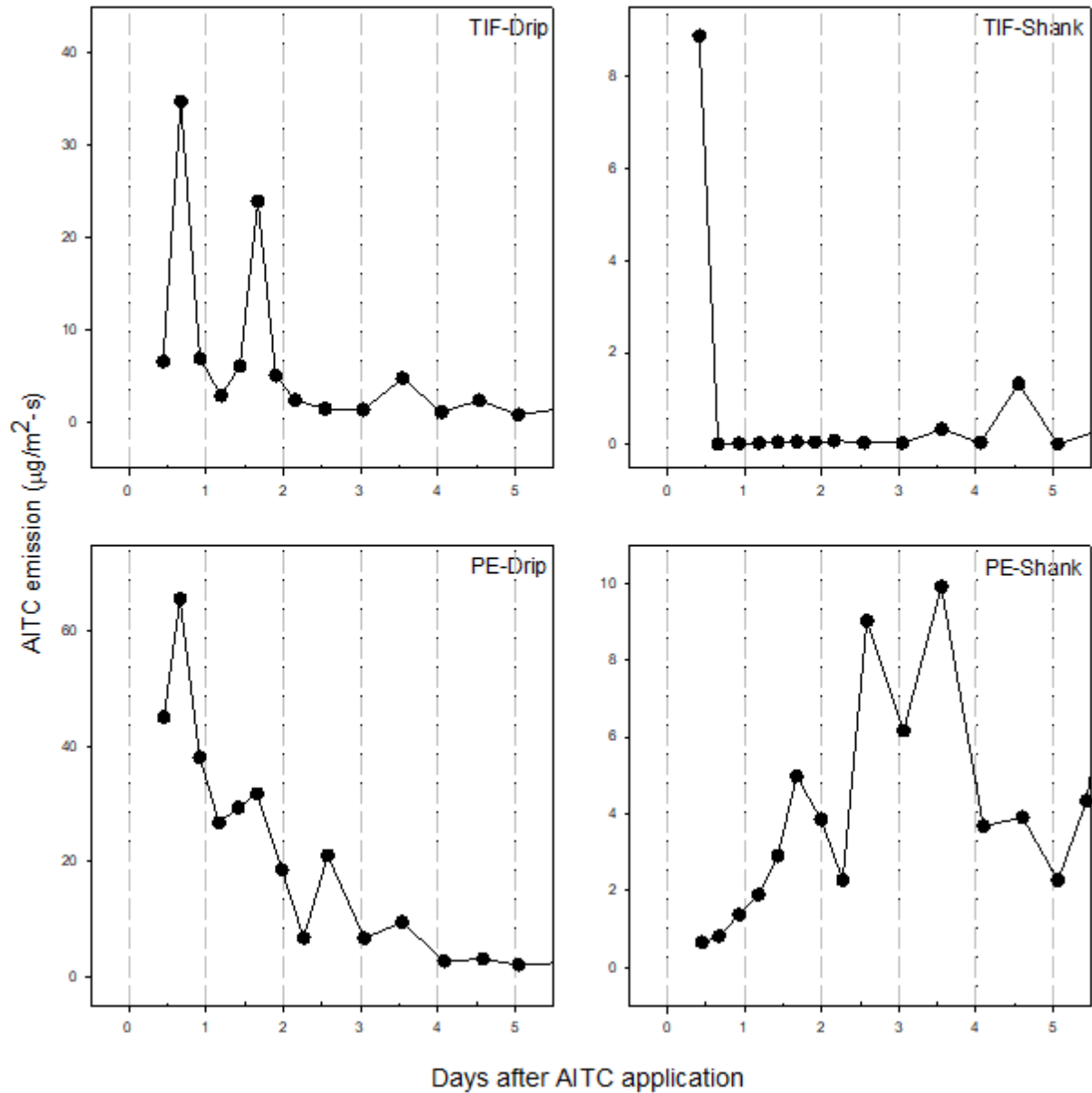
Figure 1. Allyl isothiocyanate (AITC) emissions from soil after different application methods and tarp conditions. AITC is applied through broadcast shank injection or drip irrigation, and the treated fields were covered with totally impermeable (TIF) or polyethylene (PE) film. Data were obtained from Document 50544-0008 (Ajwa et al. , 2014). The figure shows the original emissions without application rate adjustments. The figure only shows the emissions within the first 5 days which already included the maximum rates of the entire emission profiles. Five-day is also the restricted entry interval required on the Dominus® product label.
