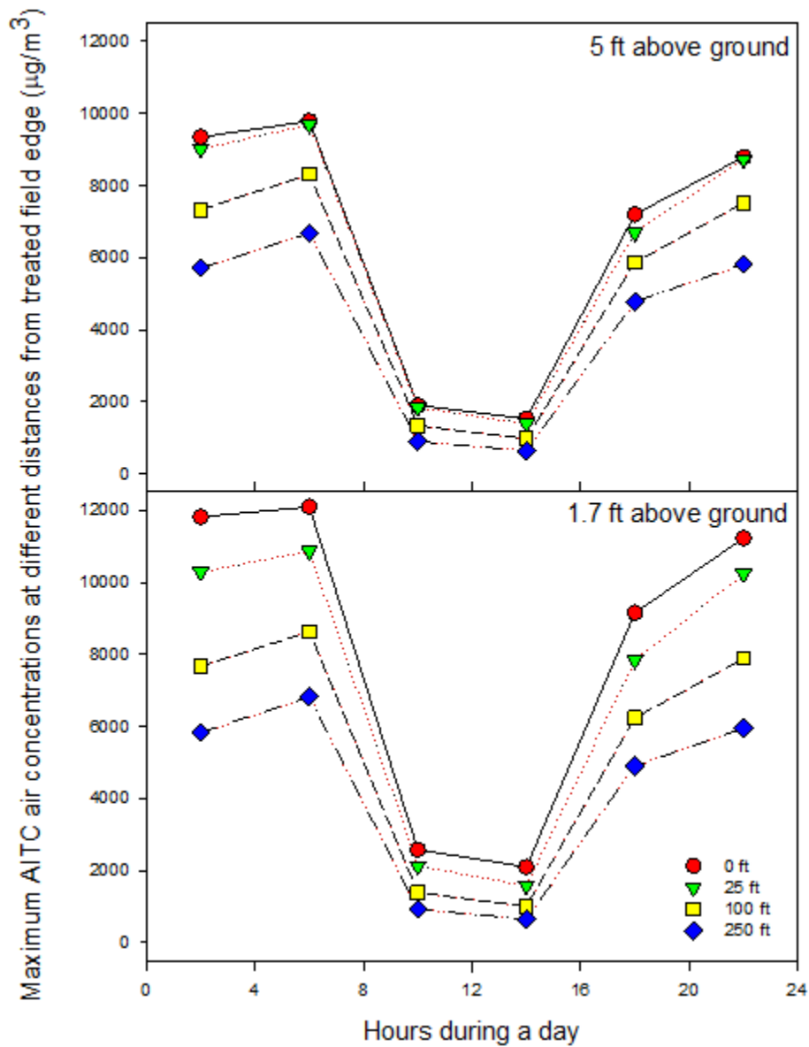
Figure 5. 4-hr averaging AITC air concentrations with different emission times. The modeled field is 40 acres and is located in Kern County. The emission rate is 100 \mu\text{g}/\text{m}^2/\text{s} flux, and the emissions occur at six different times of a day (i.e., Hour 00-04, 04-08, 08-12, 12-16, 16-20 and 20-24).
