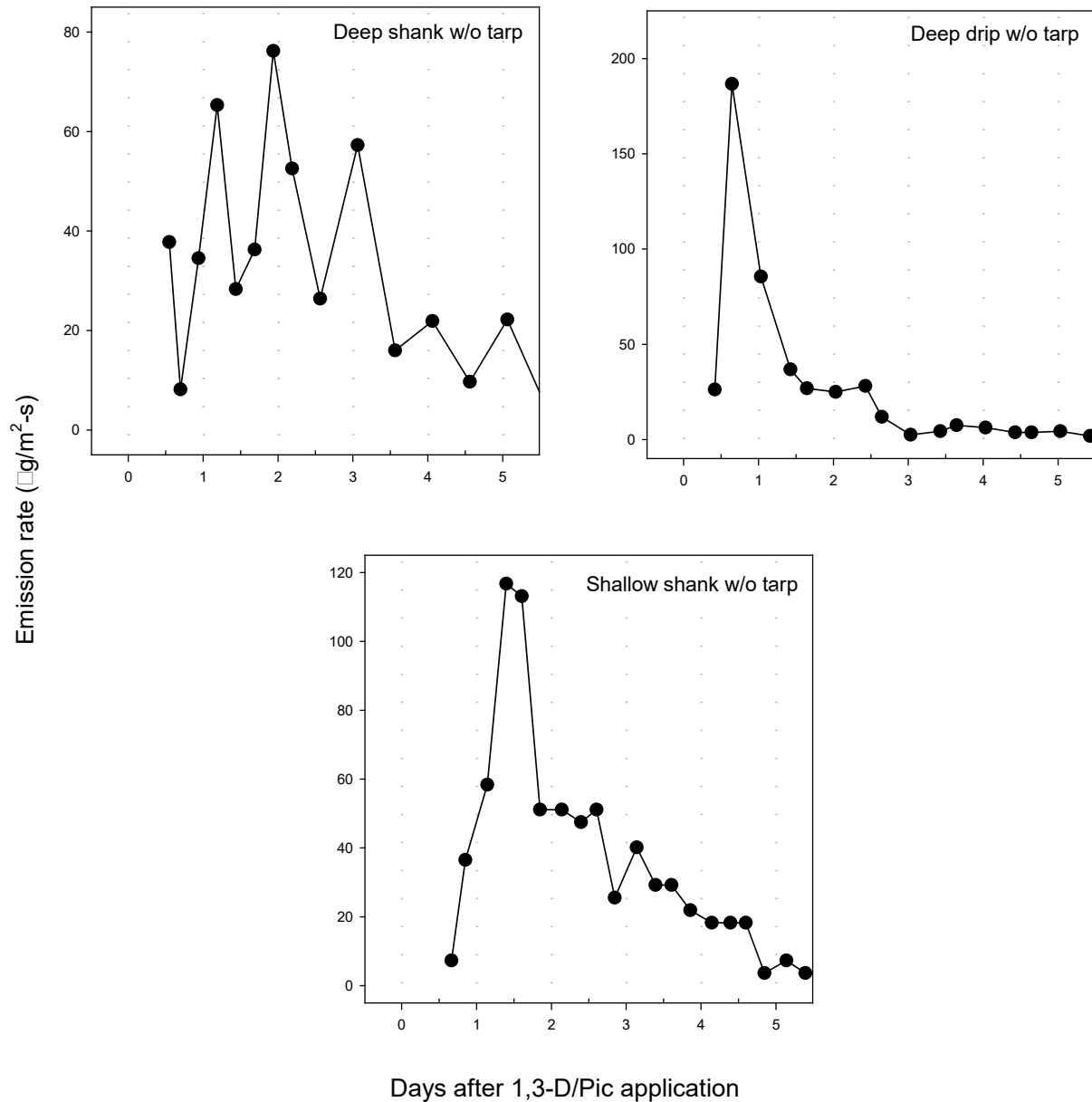
Figure 4. 1,3-Dichloropropene (1,3-D) and chloropicrin (Pic) emissions from soil. Data were obtained from various studies (Gillis, 1998; van Wesenbeeck, 1998; Ajwa, 2008). These applications were selected as surrogate data for scenarios without allyl isothiocyanate (AITC) emission data. The figure only shows the emissions within the first 5 days from the day of application. The emission rates have been normalized to 327 (for deep shank w/o tarp) or 246 (for shallow shank w/o tarp and deep drip w/o tarp) lbs/ac application rates. For shallow shank
