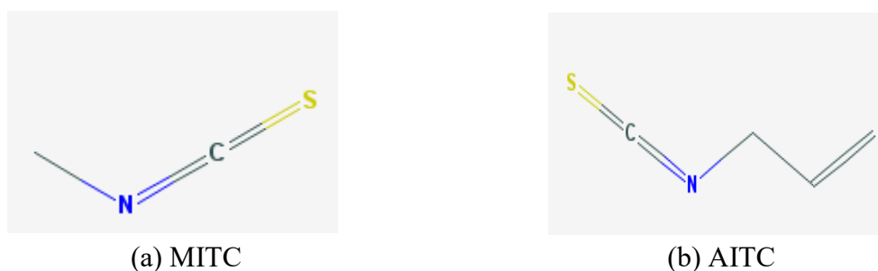
Figure 2. Structure of methyl isothiocyanate (MITC, a) and allyl isothiocyanate (AITC, b). Images are copied from PubChem (NIH, 2019).
