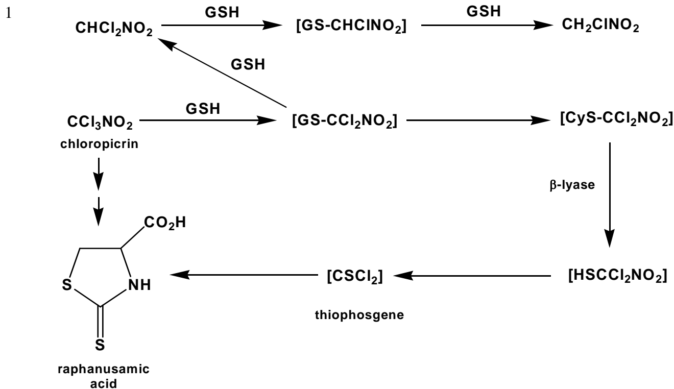
2 Figure 2. Proposed metabolism of chloropicrin in mice by dechlorination and conversion to 3 raphanusamic acid via thiophosgene (Sparks et al. , 2000).
