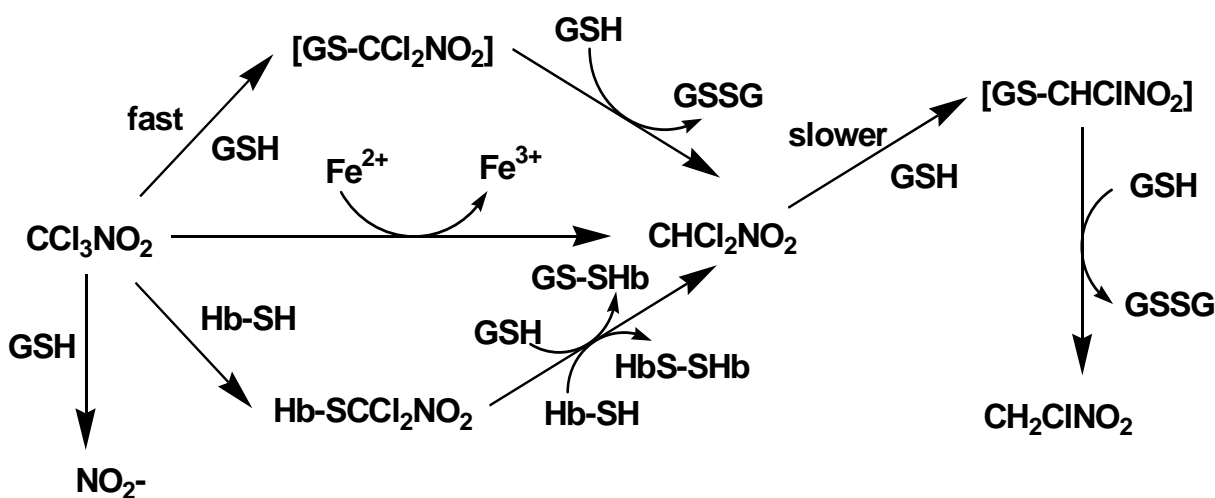
4 Figure 1. Proposed pathways for reaction of chloropicrin with glutathione and hemoglobin 5 (Sparks et al. , 1997)
