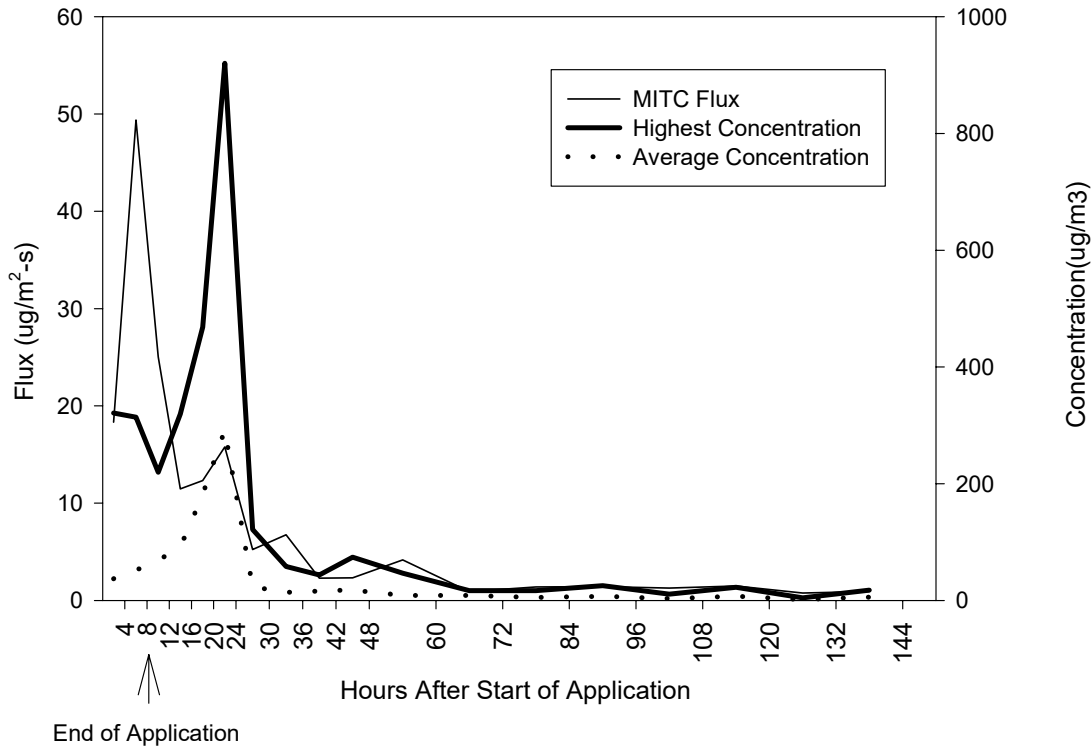
Figure 5. Fluxes and the highest measured concentration for MITC for any sampling site for each sampling interval.
