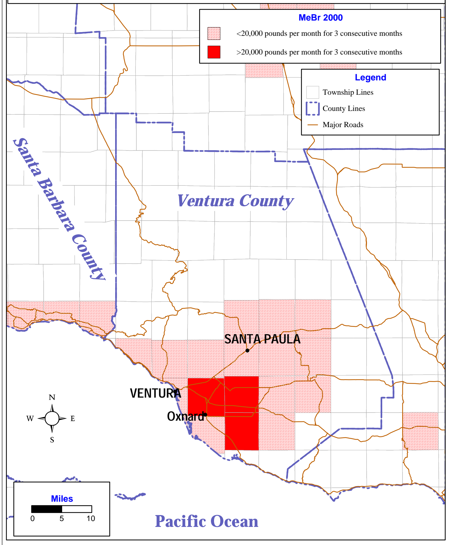
Fig 24. Methyl Bromide Use in Ventura County (2000)
