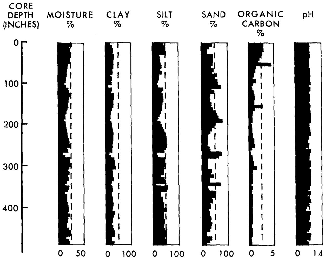
Figure 3. Soil properties to a depth of 40 feet at site 2, Ventura County.
