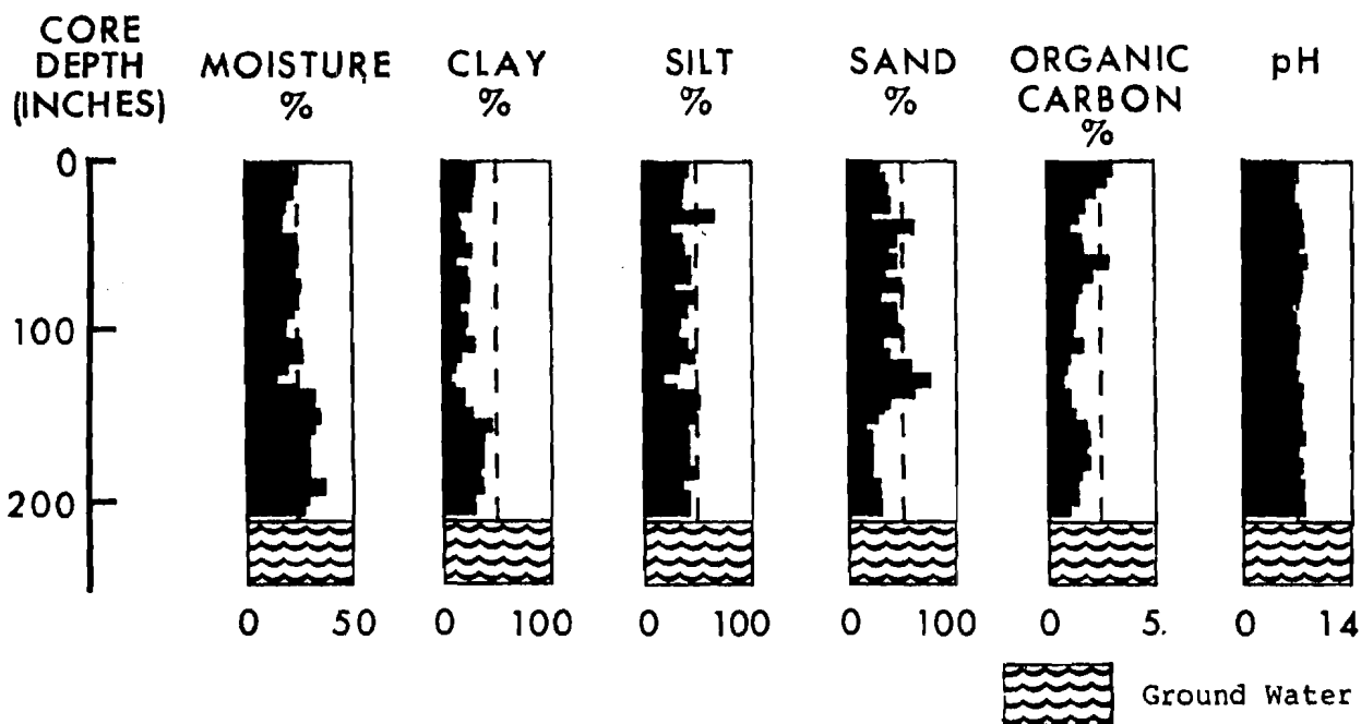
Figure 2. Soil properties to a depth of 17 feet at site 1, Ventura County.
