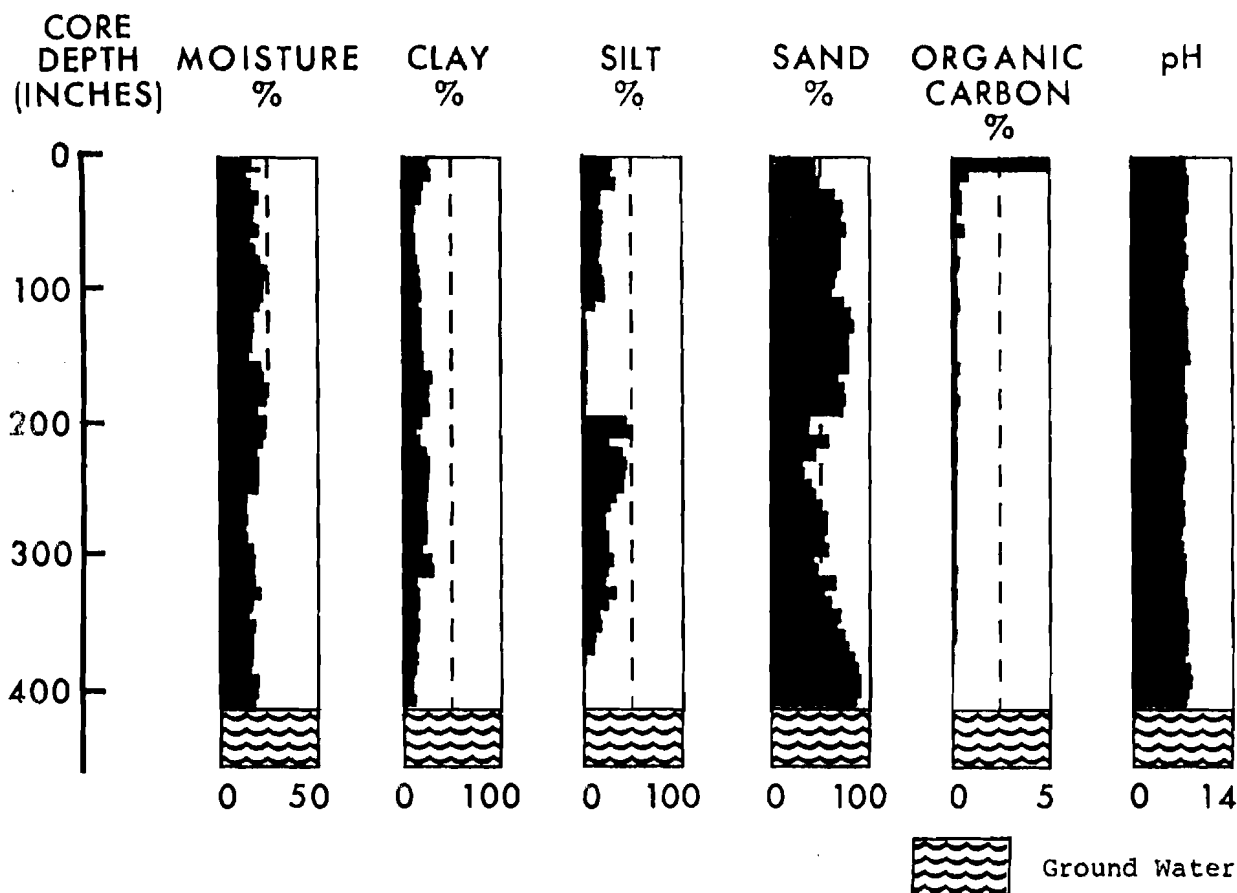
Figure 5. Soil properties to a depth of 28 feet at site 4, Tulare County.
