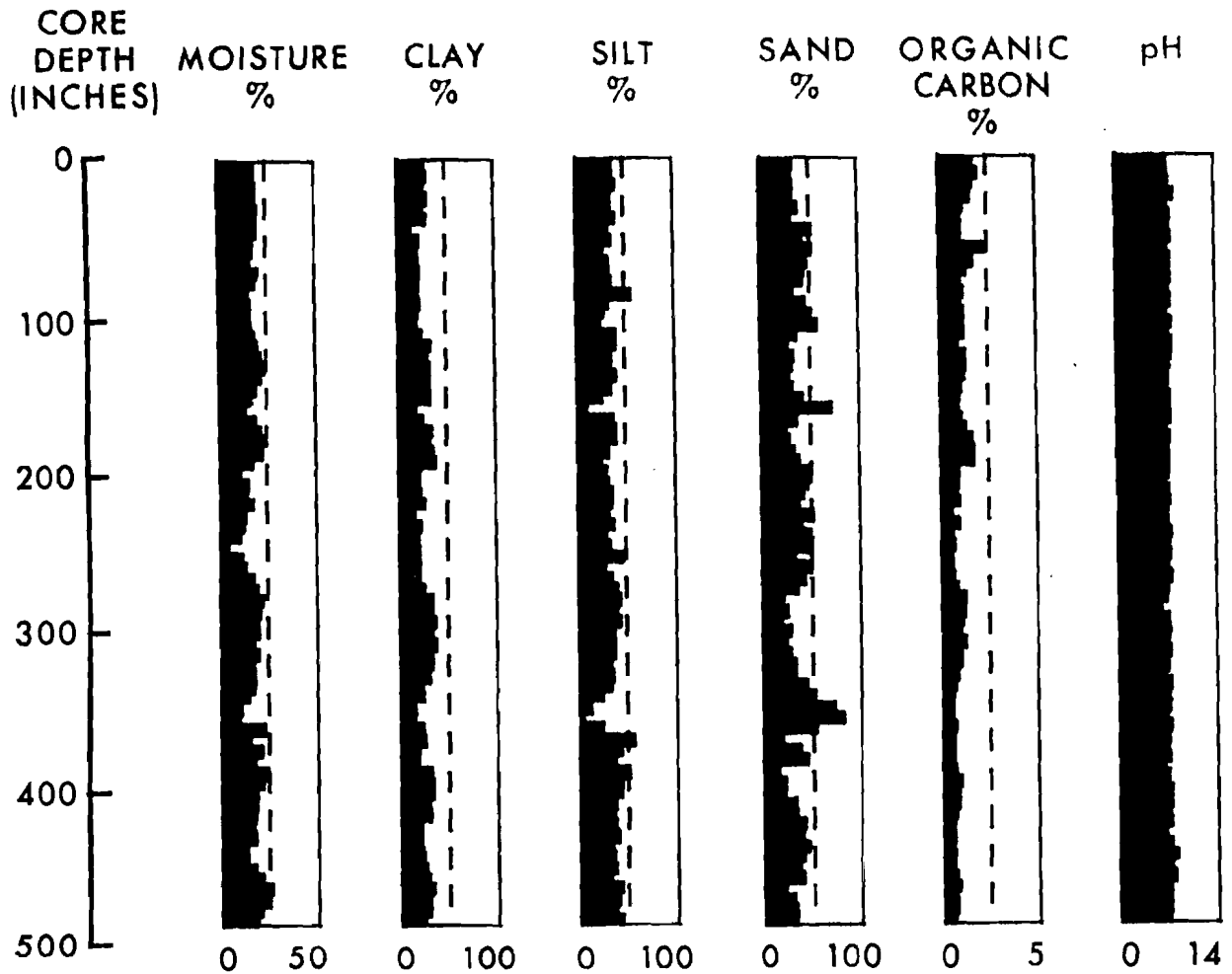
Figure 4. Soil properties to a depth of 40 feet at site 3, Ventura County.
