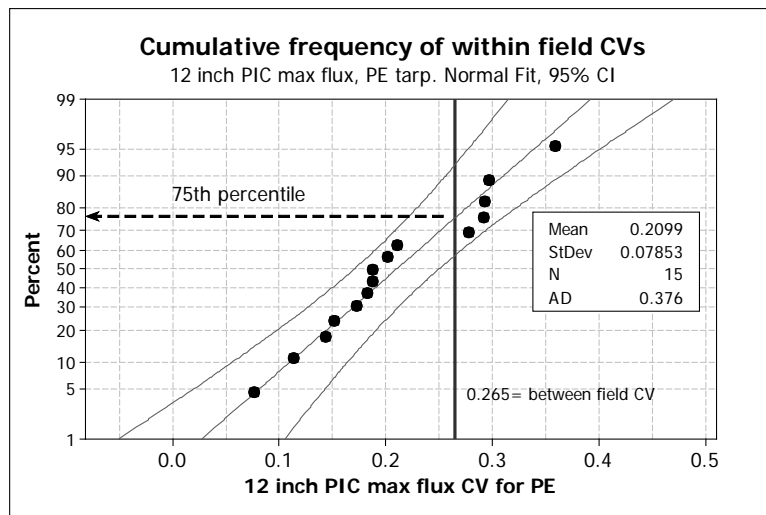
Figure 1. Comparison of within- and between-max flux CV for 12 inch PIC application with PE tarp. Max flux ( \text{ug m}^{-2} \text{sec}^{-1} ) expressed on 100 \text{ lbs ac}^{-1} applied basis.
