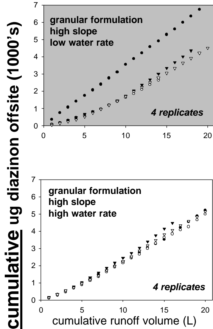
Figure 7b. Mean runoff profiles (mean conc. +/- sd vs. volume) and cumulative mass vs. volume curves for granular, high slope, low water rate treatment group (plots 1, 10, 20, 25) and granular, high slope, high water rate groups (plots 3,9,18,27)
