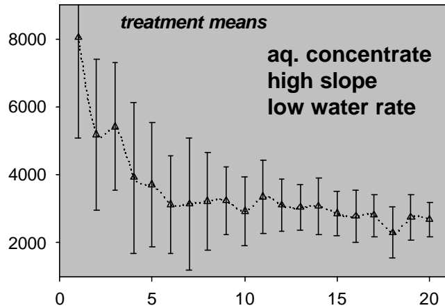
Figure 7d. Mean runoff curves (mean conc. +/- sd vs. volume) AND cumulative mass vs. volume curves for aqueous concentrate, high slope, low water rate treatment group (plots 4, 11, 17, 26) and aqueous, high slope, high water rate groups (plots 2, 12, 19, 28)
