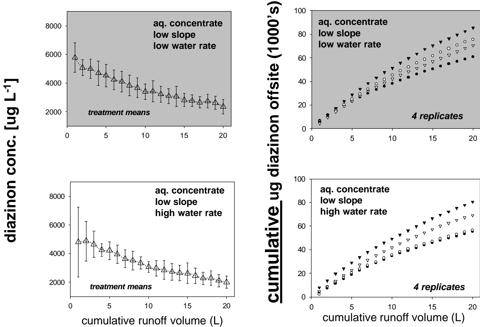
Figure 7c. Mean runoff curves (mean conc. +/- sd vs. volume) AND cumulative mass vs. volume curves for aqueous concentrate, low slope, low water rate treatment group (plots 5, 16, 22, 32) and aqueous concentrate, low slope, high water rate groups (plots 8,14,24,29)
