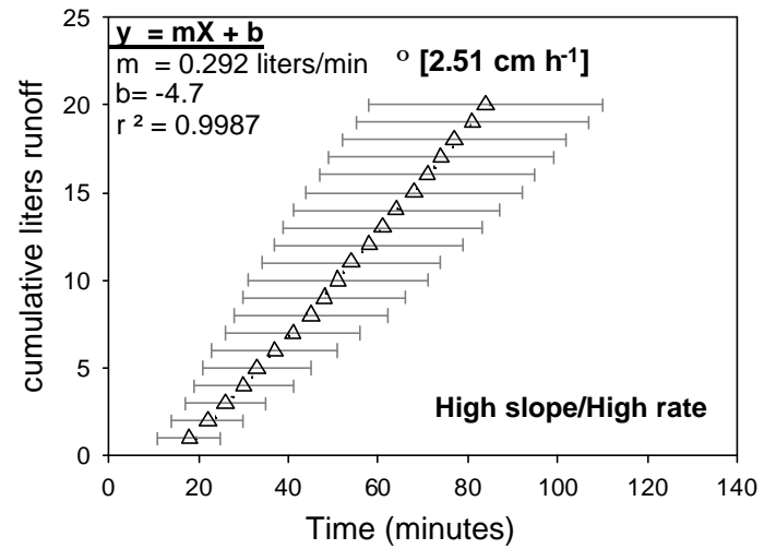
Figure 3. Treatment mean cumulative water runoff curves: cumulative runoff volume vs. mean time. Samples were collected in 1-L increments; The time (+/- SD) is the mean of all 8 plots in the respective water application rate/slope treatment group. The low and high water application rates were 3.18 cm h -1 and 4.88 cm h -1 , respectively, and the low and high slopes were 2.5% and 5%, respectively.
