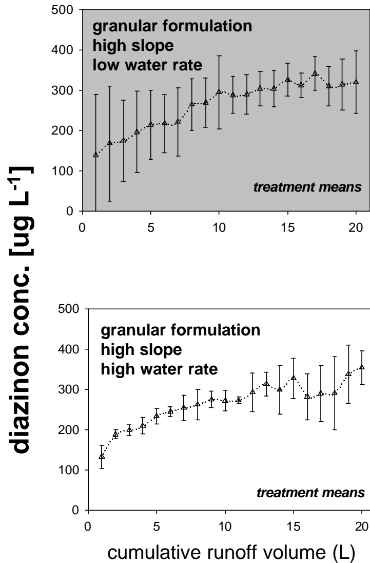
Figure 7b. Mean runoff profiles (mean conc. +/- sd vs. volume) and cumulative mass vs. volume curves for granular, high slope, low water rate treatment group (plots 1, 10, 20, 25) and granular, high slope, high water rate groups (plots 3,9,18,27)
